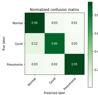
(b) Confusion Matrix normalization
