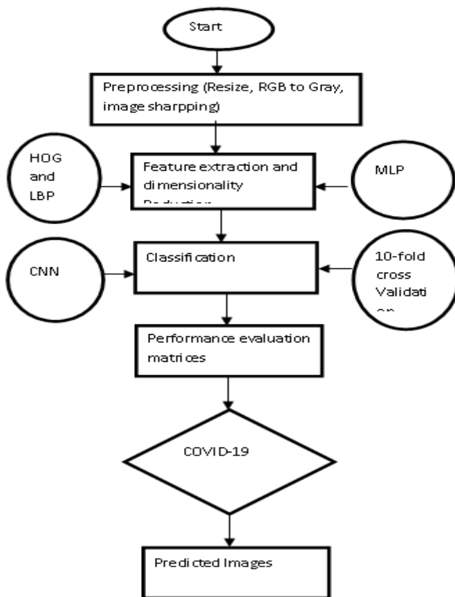
Figure 2: Flowchart of Proposed Model
