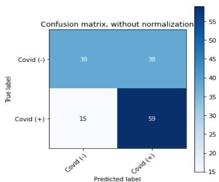
(a) Confusion Matrix without normalization
