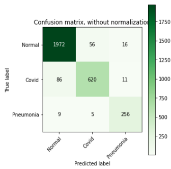
(a) Confusion Matrix without normalization
