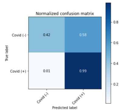
(a) normalization of a confusion matrix
