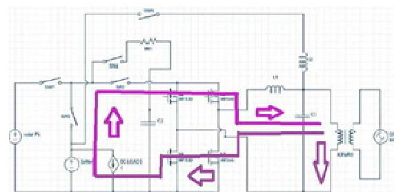
Figure 5. Battery to Grid
