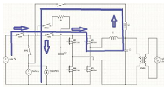
Figure 4. PV to Battery Charging
