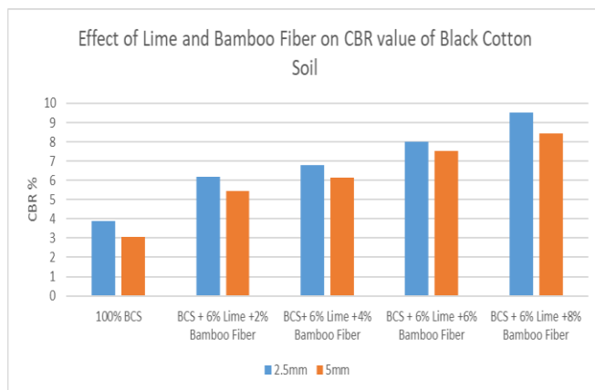
Graph No.-10 Graphical representation of CBR Values of BC Soil Blend by 6% Lime with Various percentage of Bamboo Fiber
