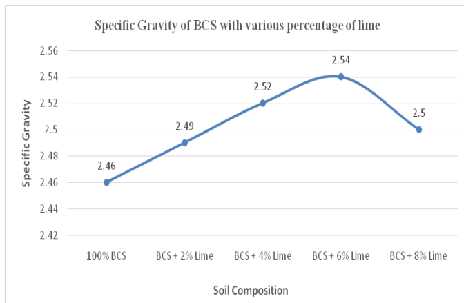
Graph No-03 Graphical Representation of BCS with various percentage of lime
