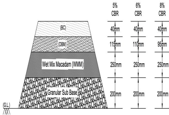
Figure- 22 Pavement composition with thickness of each layer for Different CBR values
