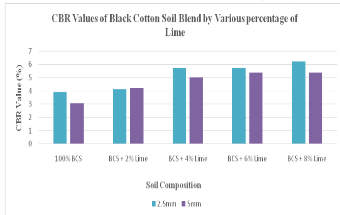
Graph No-07. Graphical representation of CBR Values of BCS Blend by Various percentage of Lime
