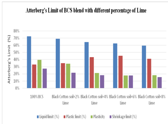
Graph No.-02 Graphical comparison of Atterberg's Limits of BCS blend with different percentage of Lime
