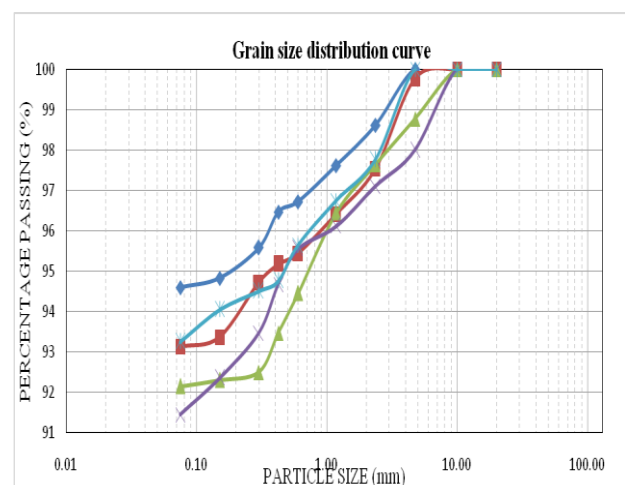
Graph.1 Grain size distribution curve for black cotton soil
