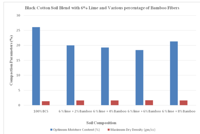
Graph No-08 Graphical Variation of OMC and MDD of BCS with 6% Lime and various percentage of Bamboo Fibers
