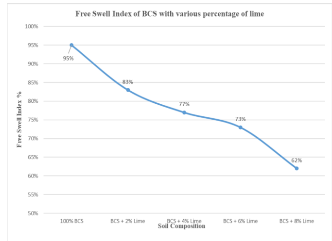
Graph No.-04 Graphical Representation of Free Swell Index of BCS with various percentage of lime
