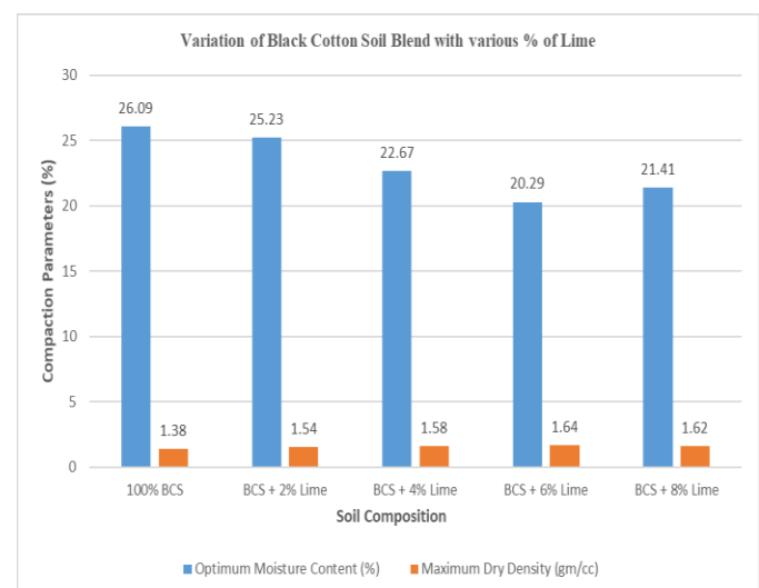
Graph No.-05 Graphical Variation of OMC and MDD of BCS with various percentage of lime
