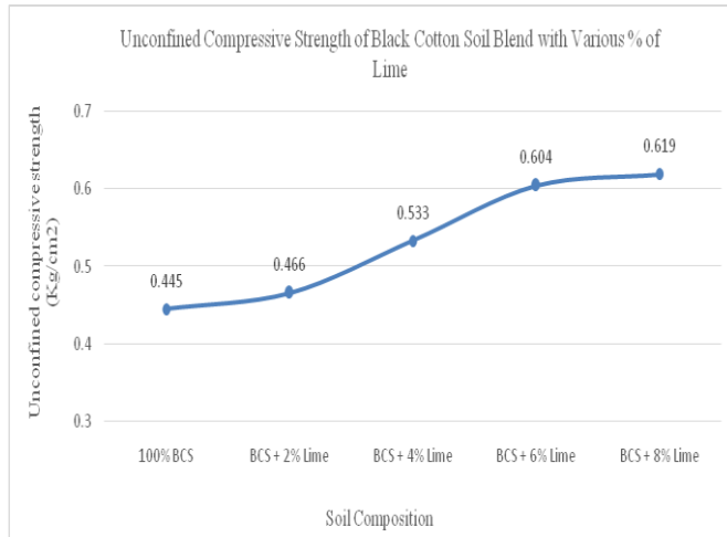
Graph-06 Graphical representation of UCS of BCS Blend with Various percentage of Lime
